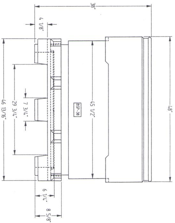
SIDE ELEVATION
