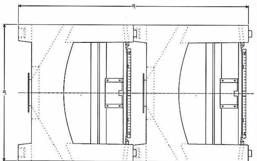
TOP VIEW WITH DUST COVER LID REMOVED
