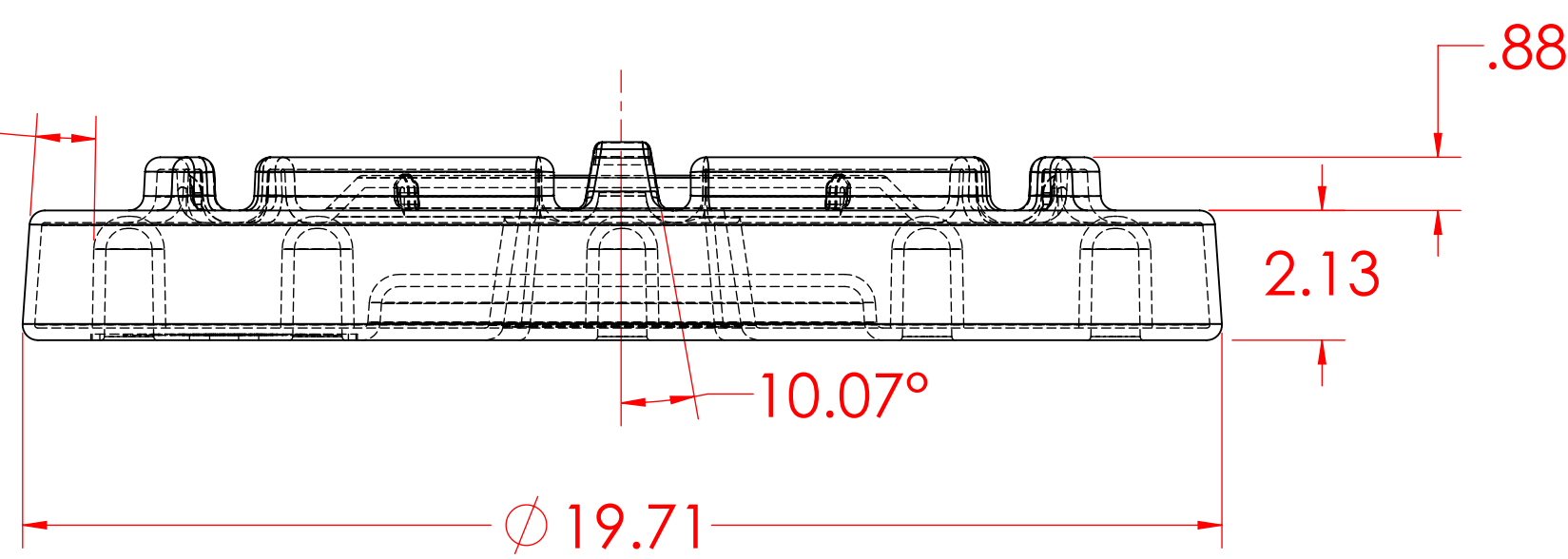
SECTION L-L
