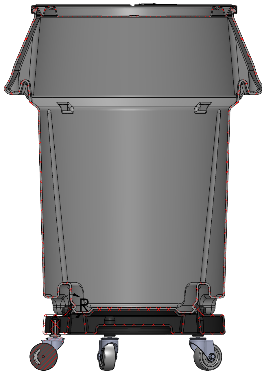
SECTION P-P
